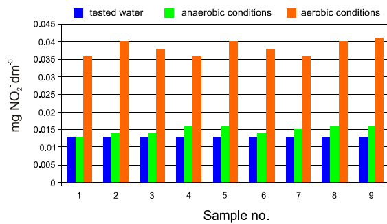
Fig. 3. The effect of oxygen access on the release of nitrites from Lake Góreckie bottom sediments.
