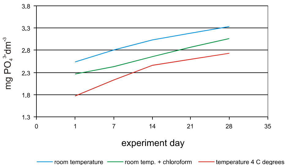
Fig. 5. The effect of temperature on the release of orthophosphates from Lake Góreckie bottom sediments.
