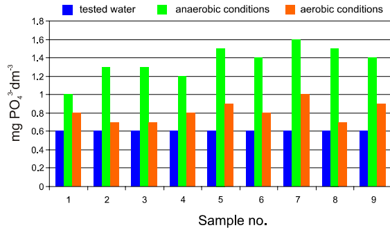
Fig. 1. The effect of oxygen access on the release of orthophosphates from Lake Góreckie bottom sediments.
