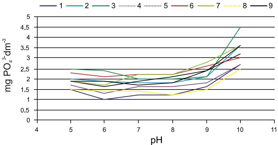
Fig. 4. The effect of water pH on the release of orthophosphates from Lake Góreckie bottom sediments.
