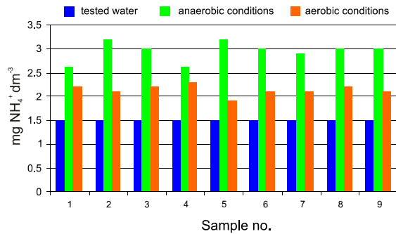
Fig. 2. The effect of oxygen access on the release of ammonium nitrogen from Lake Góreckie bottom sediments.
